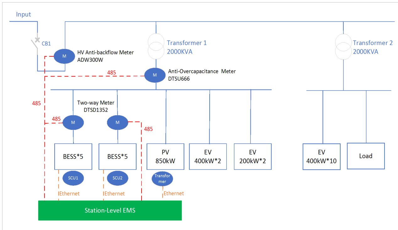
Fig. 1 Single Line Diagram of the System
