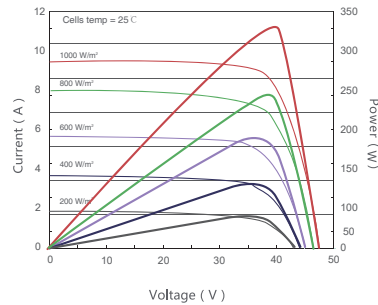
Current-Voltage & Power-Voltage Curves (330W)
