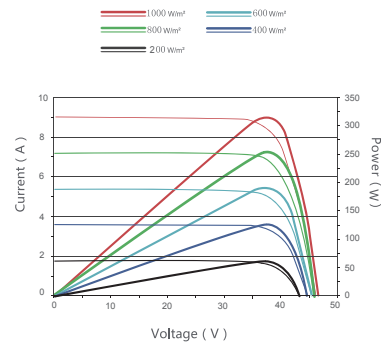
Current-Voltage & Power-Voltage Curves (310W)
