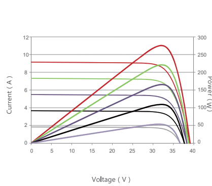
Current-Voltage & Power-Voltage Curves (275W)
